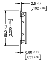
QUICK CONNECT TERMINAL 90° BENT
